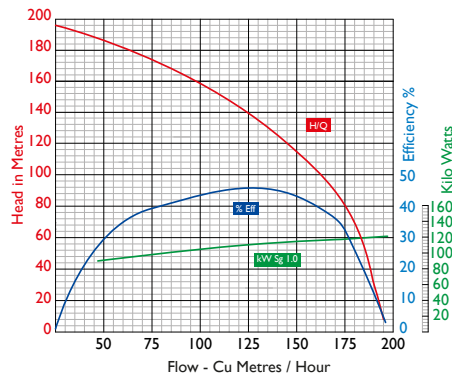
150 DWHH 150kW, 1450 RPM (50Hz) Three Stage Pump
